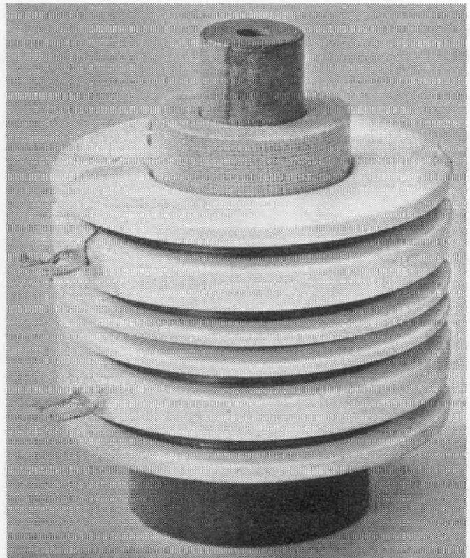
FIGURE 3. One of the low frequency coils showing construction
