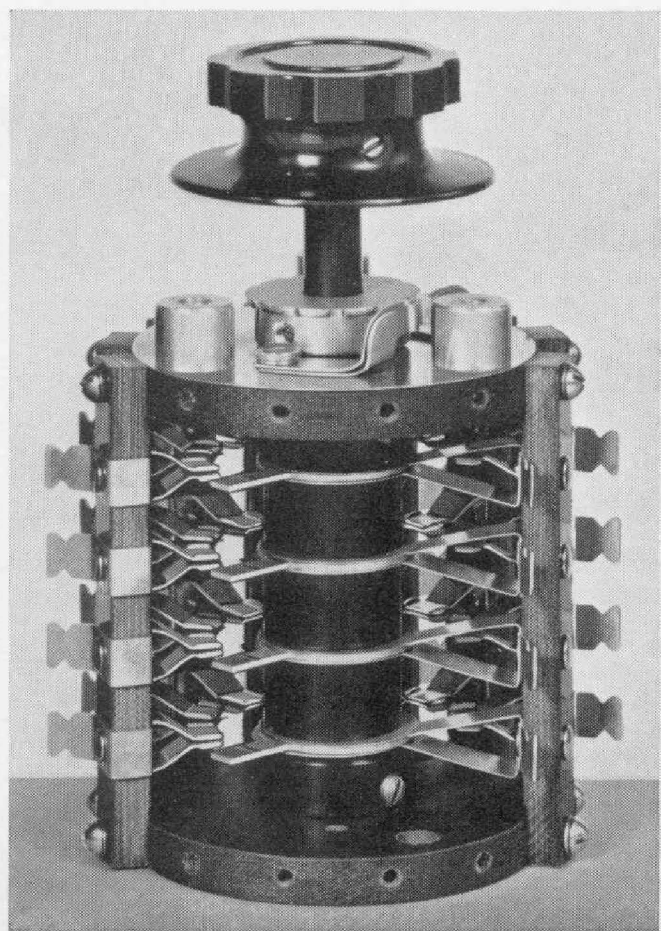
FIGURE 5. Construction of the band-change switch
