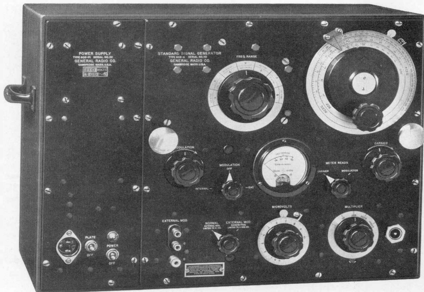
FIGURE 1. Panel view of the TYPE 605-A Standard-Signal Generator
