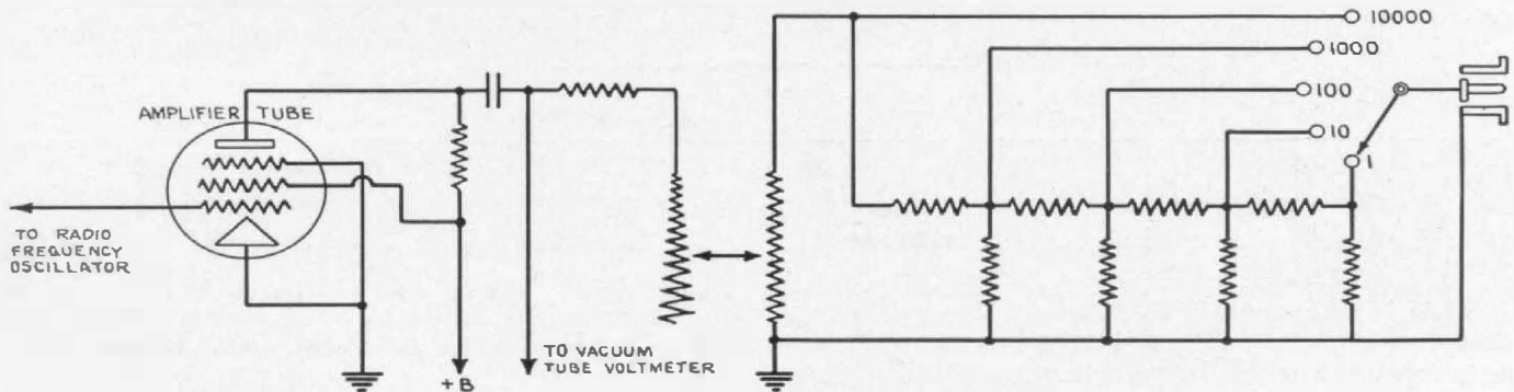
FIGURE 7. Schematic diagram of the output system
